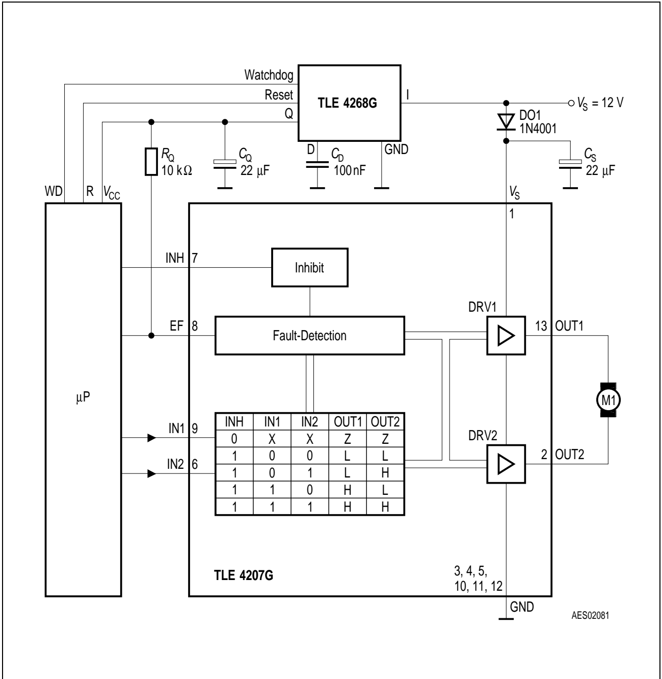
Figure 3 Application Circuit
