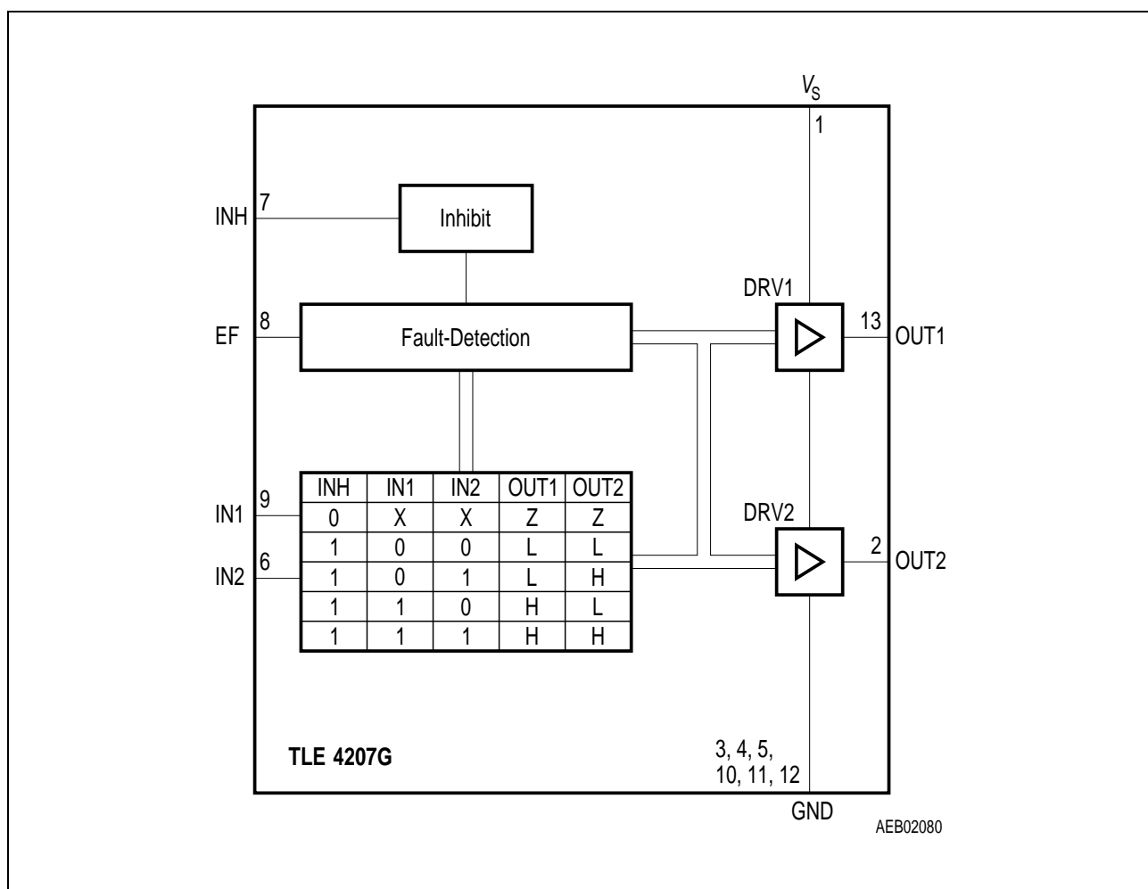
Figure 2 Block Diagram
